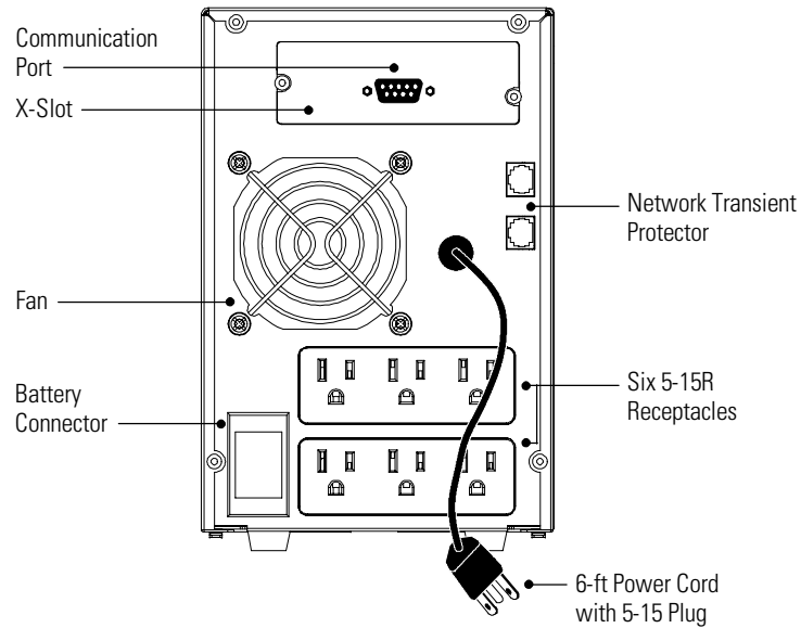
Figure 3. PW5125 1000 and PW5125 1500 Rear Panel
