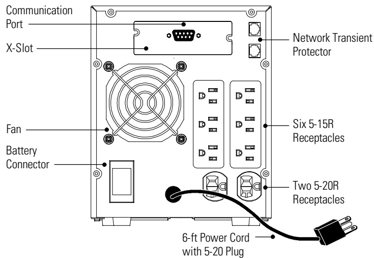
Figure 4. PW5125 2200 Rear Panel
