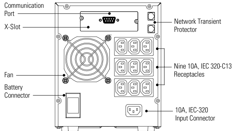
Figure 6. PW5125 2200i Rear Panel
