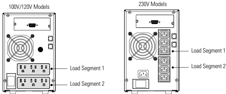
Figure 17. 1000 VA and 1500 VA Load Segments
