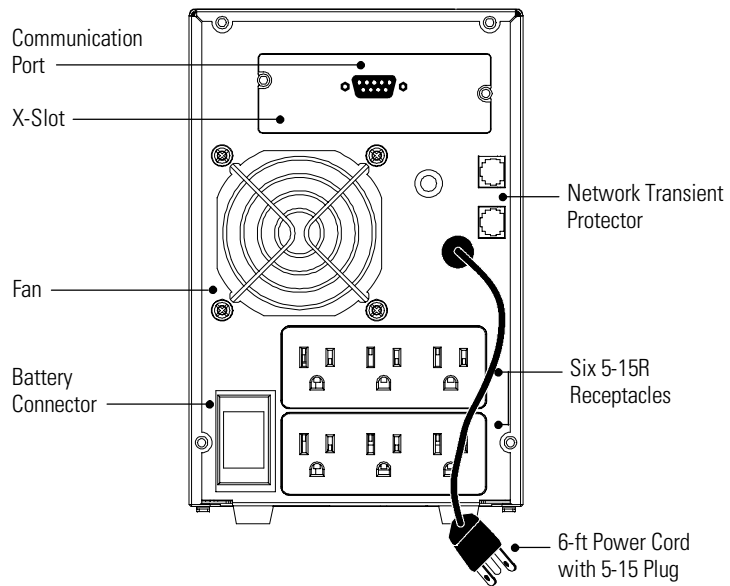
Figure 7. PW5125 1000j Rear Panel
