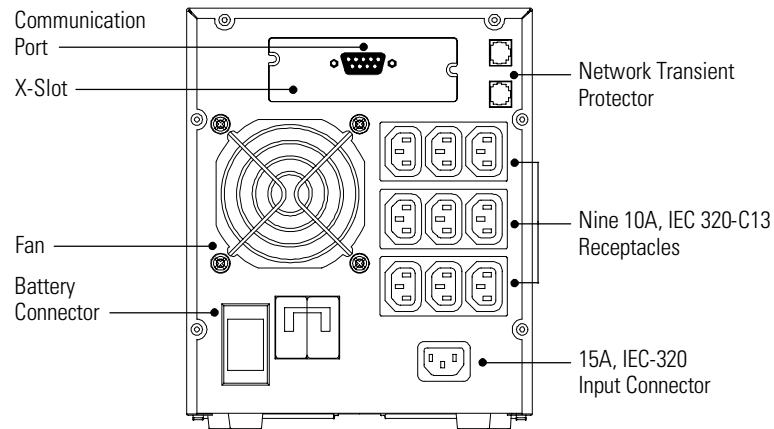
Figure 10. PW5125 2200b Rear Panel
