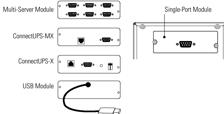
Figure 14. Optional X-Slot Modules
