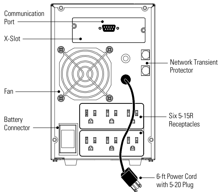
Figure 8. PW5125 1500j Rear Panel
